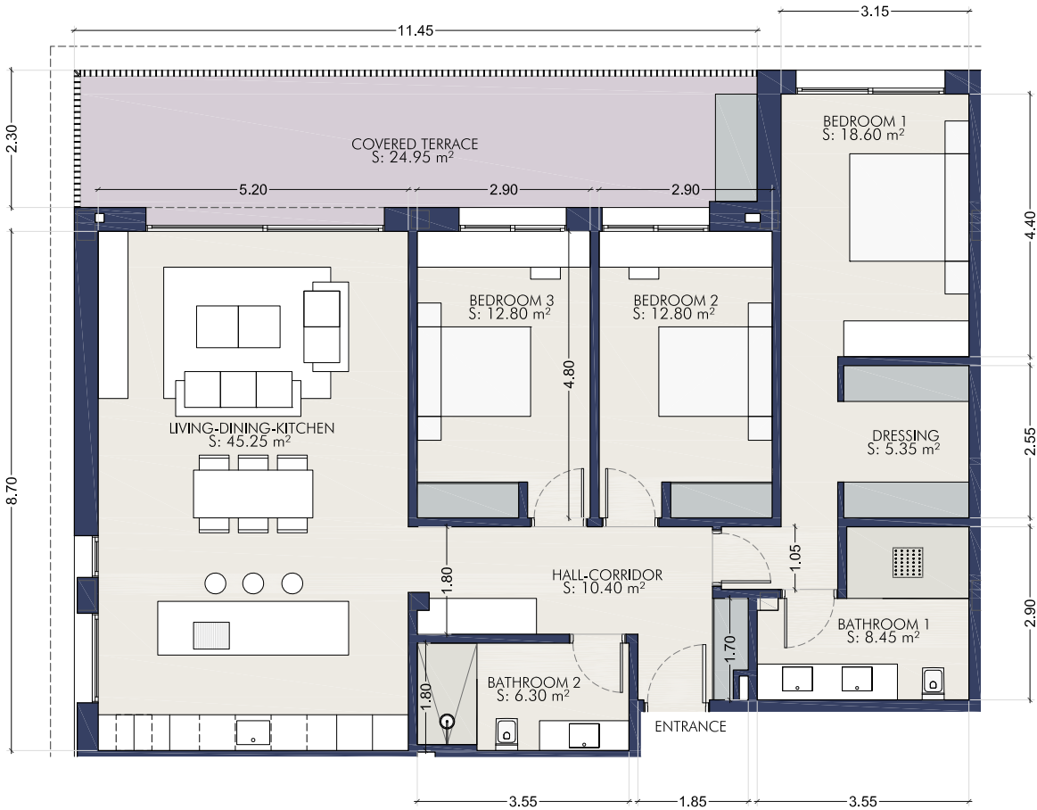
Ground Floor
