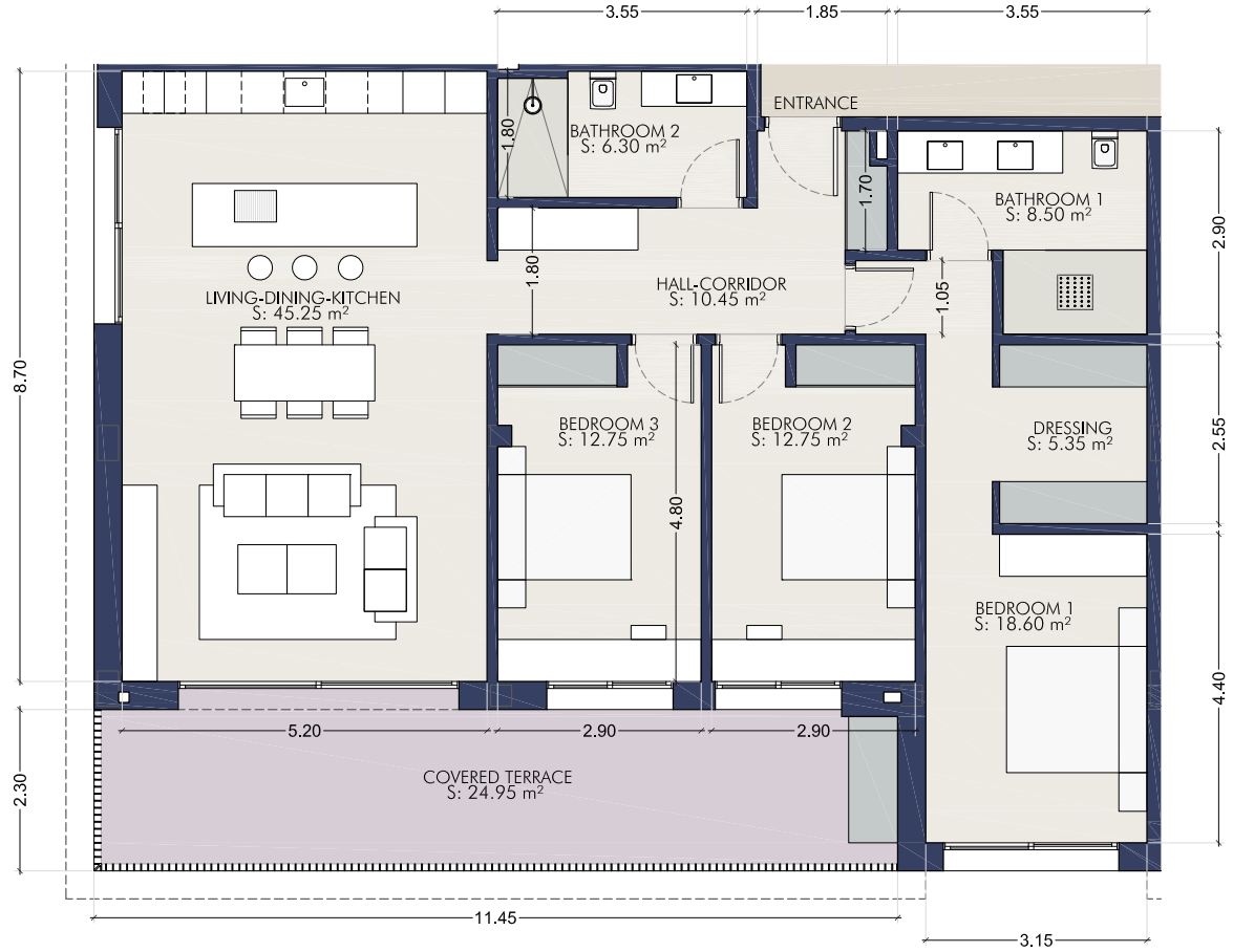
Ground Floor
