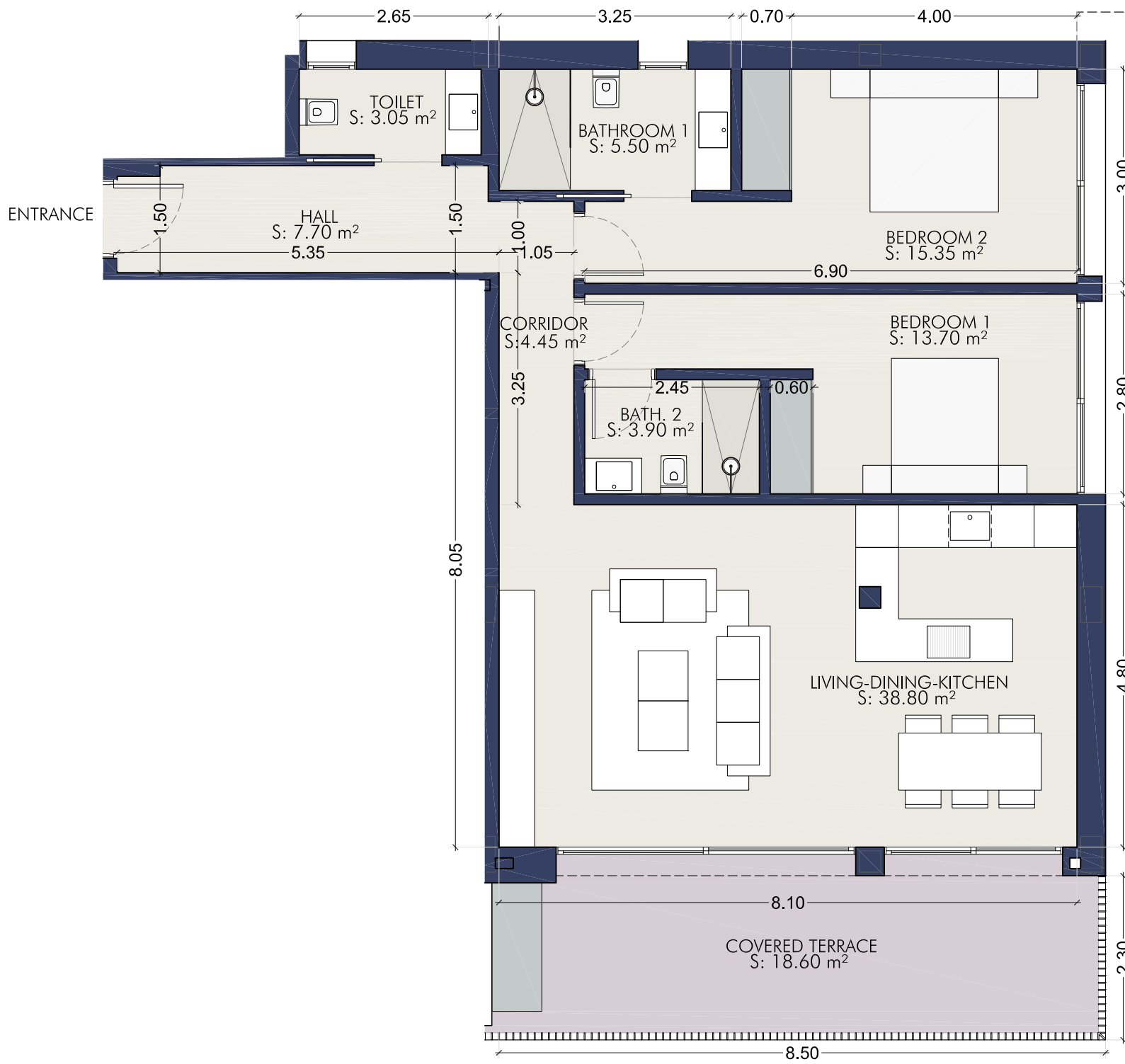
Ground Floor
