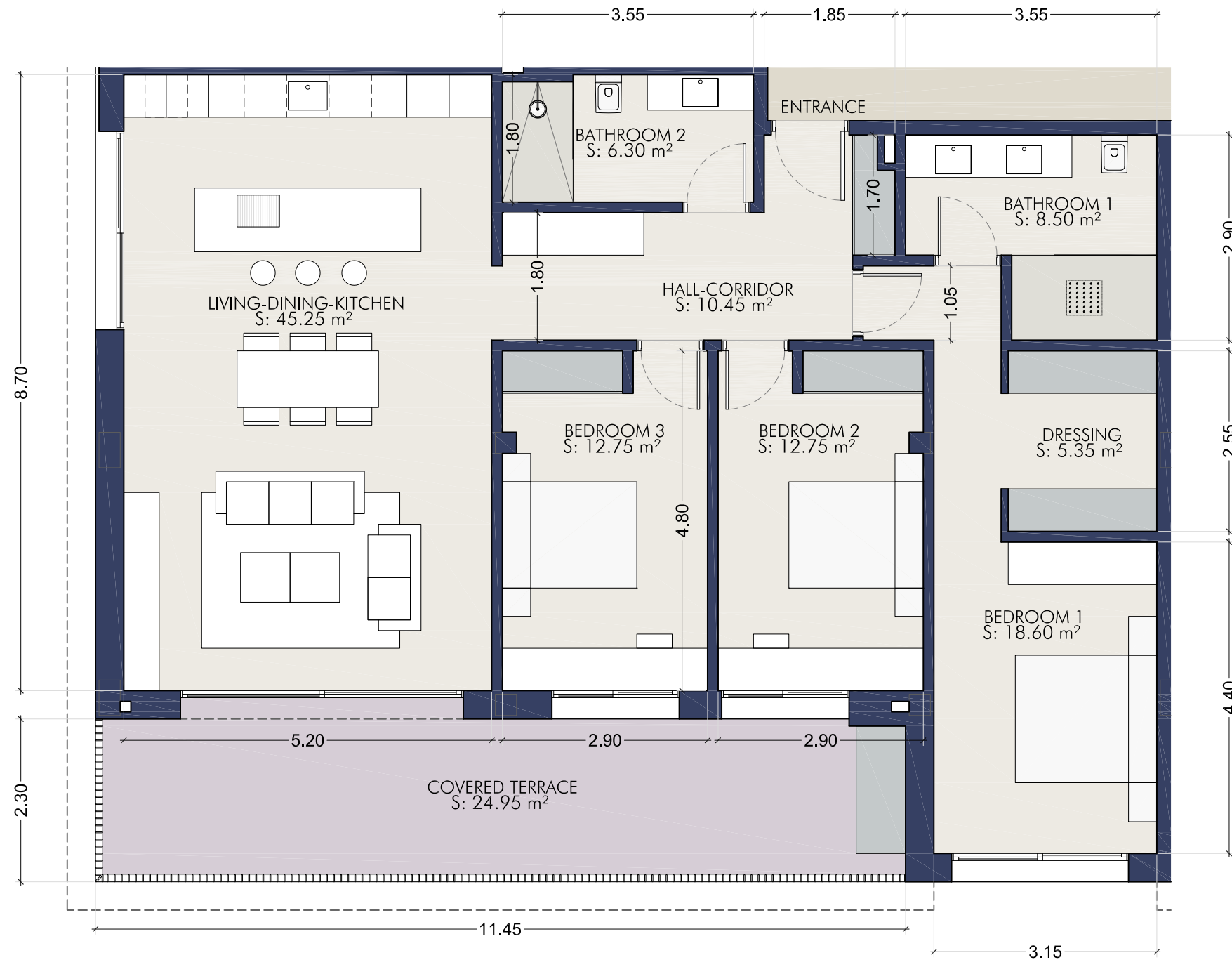
Ground Floor
