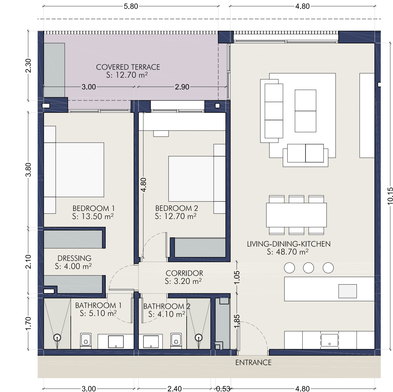
Ground Floor
